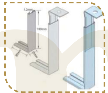
Adjustable Head (Restraint IAHR)
